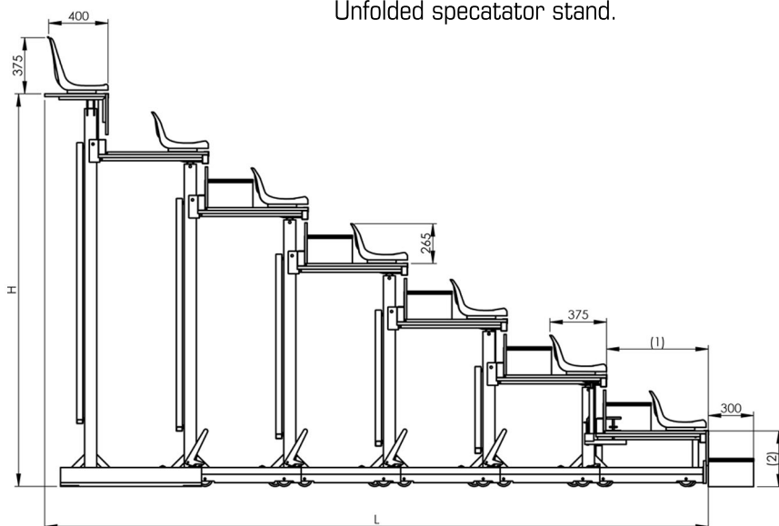
Unfolded spectator stand.
